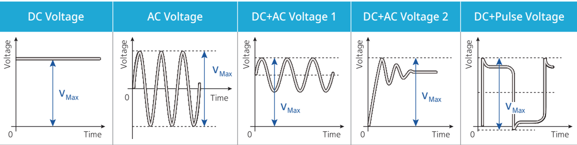
Types of Voltage Applied to the Capacitor
